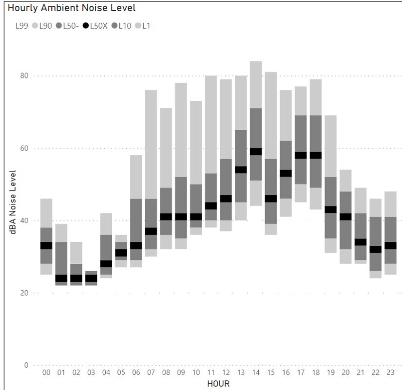
Figure 4-2 Site Specific Ambient Noise Measurement Results Moulton January 4, 2020
