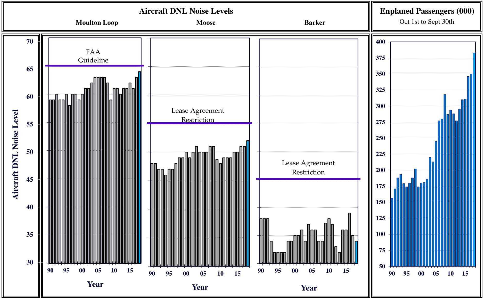
Figure 4-12 2018 Annual DNL Noise Report Jackson Hole Airport 2018 Annual Report October 1st 2017 to September 30th 2018
