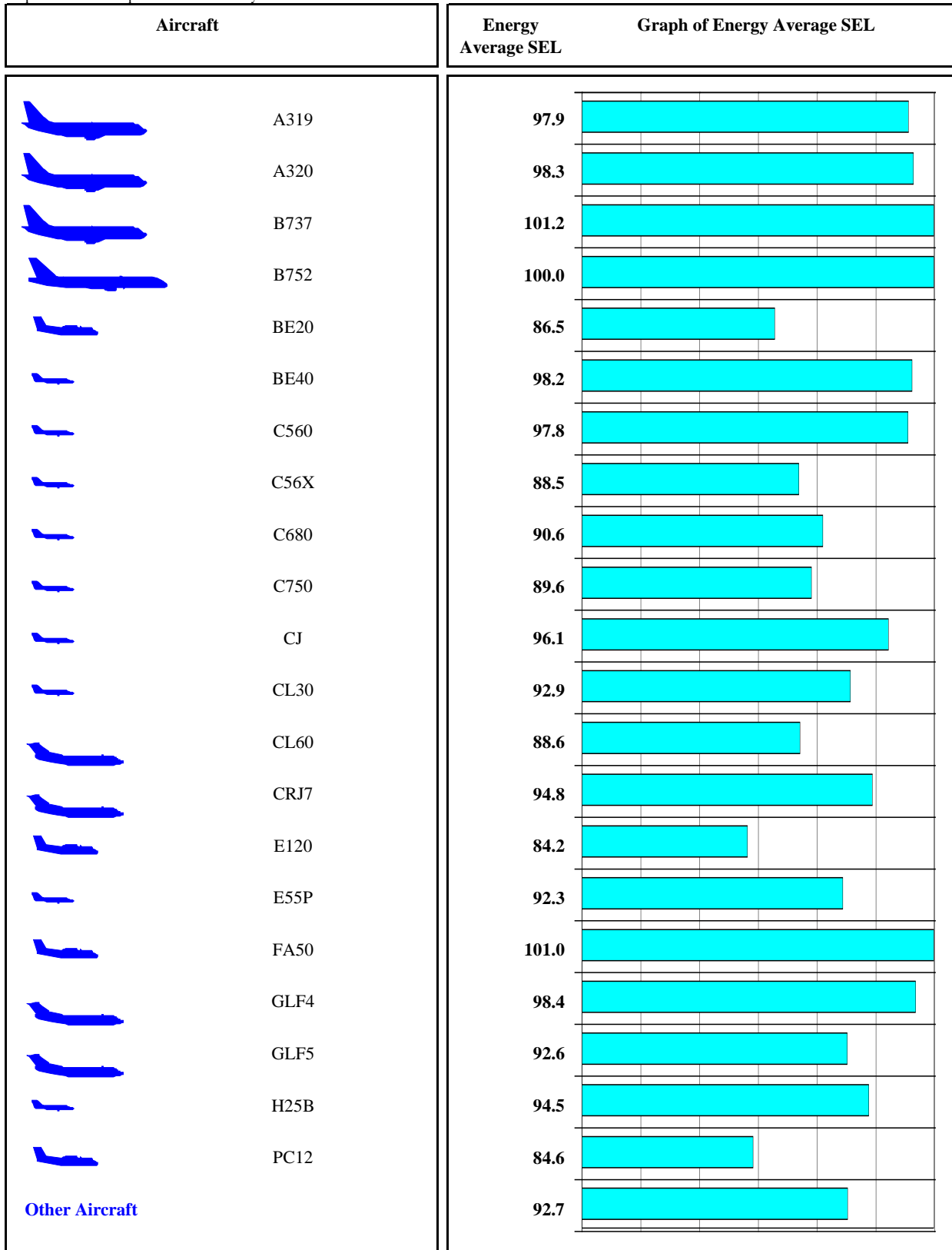
Figure 4-6 Single Event Noise Level by Aircraft Report Jackson Hole Airport 2018 Annual Report Period: June 30, 2018 to July 13, 2018 Site: Moulton Loop - Zenith Drive and Spring Gulch Road Operations: Departure Runway: 19 Tracks: ALL
