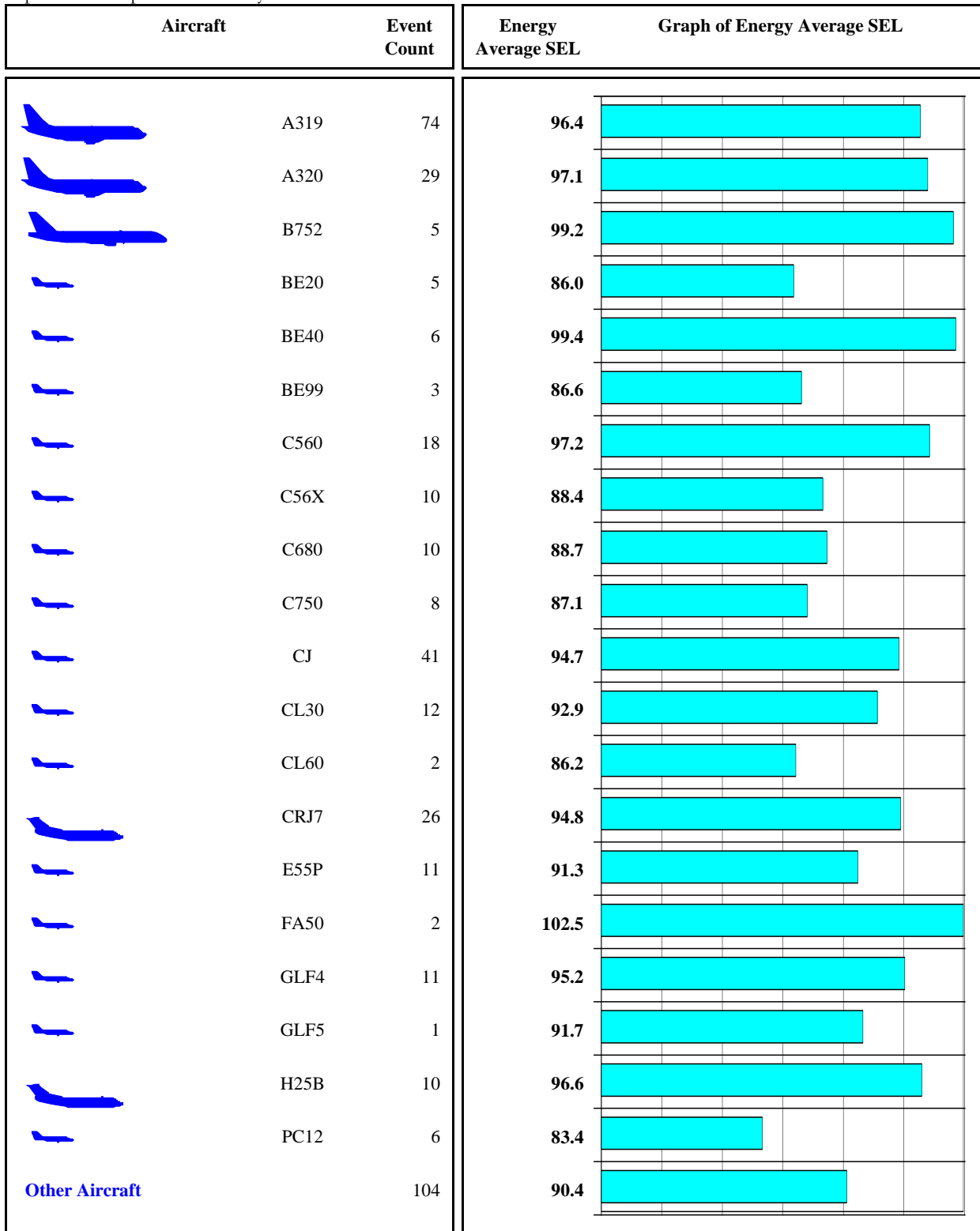
Figure 4-6 Single Event Noise Level by Aircraft Report Jackson Hole Airport 2016 Annual Report Period: August 30, 2016 to September 12, 2016 Site: Moulton Loop - Zenith Drive and Spring Gulch Road Operations: Departure Runway: 19 Tracks: ALL
