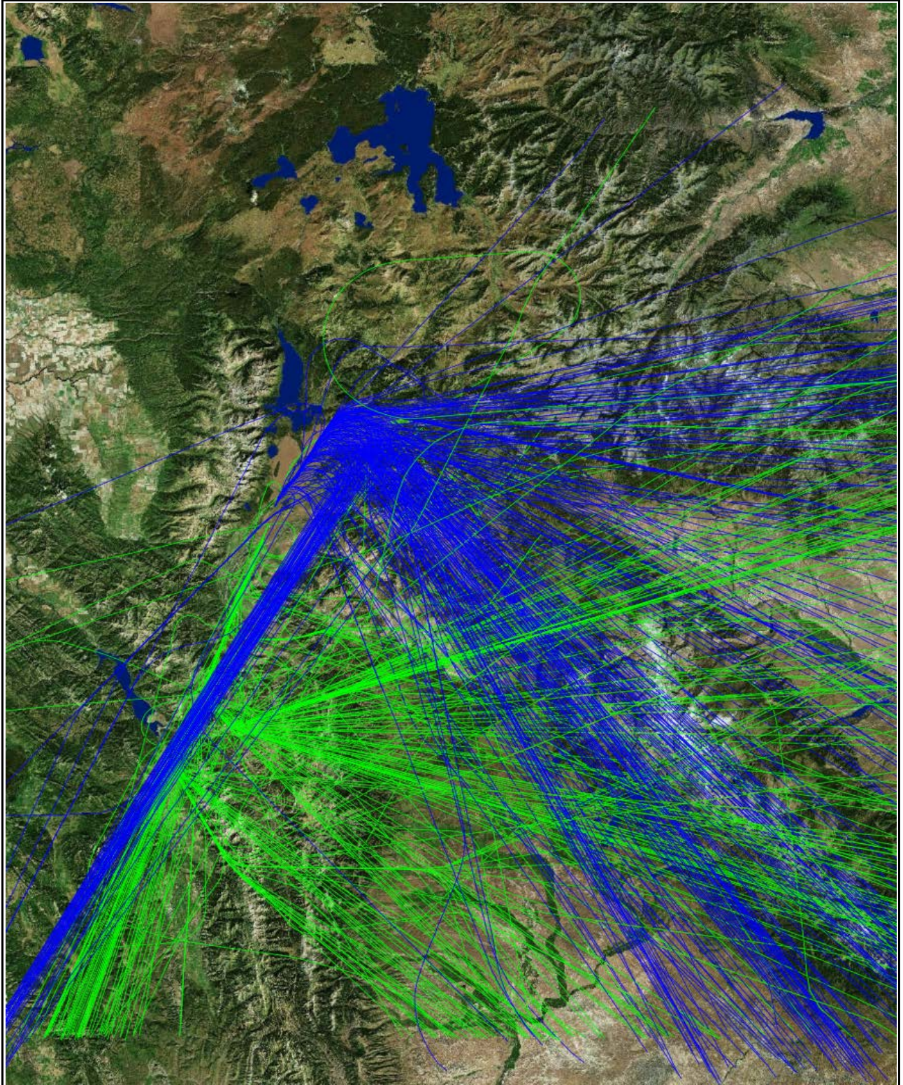
Figure 5-2 Flight Tracks for North Flow Jackson Hole Airport 2016 Annual Report Arrival and Departure Tracks for Runway 01
