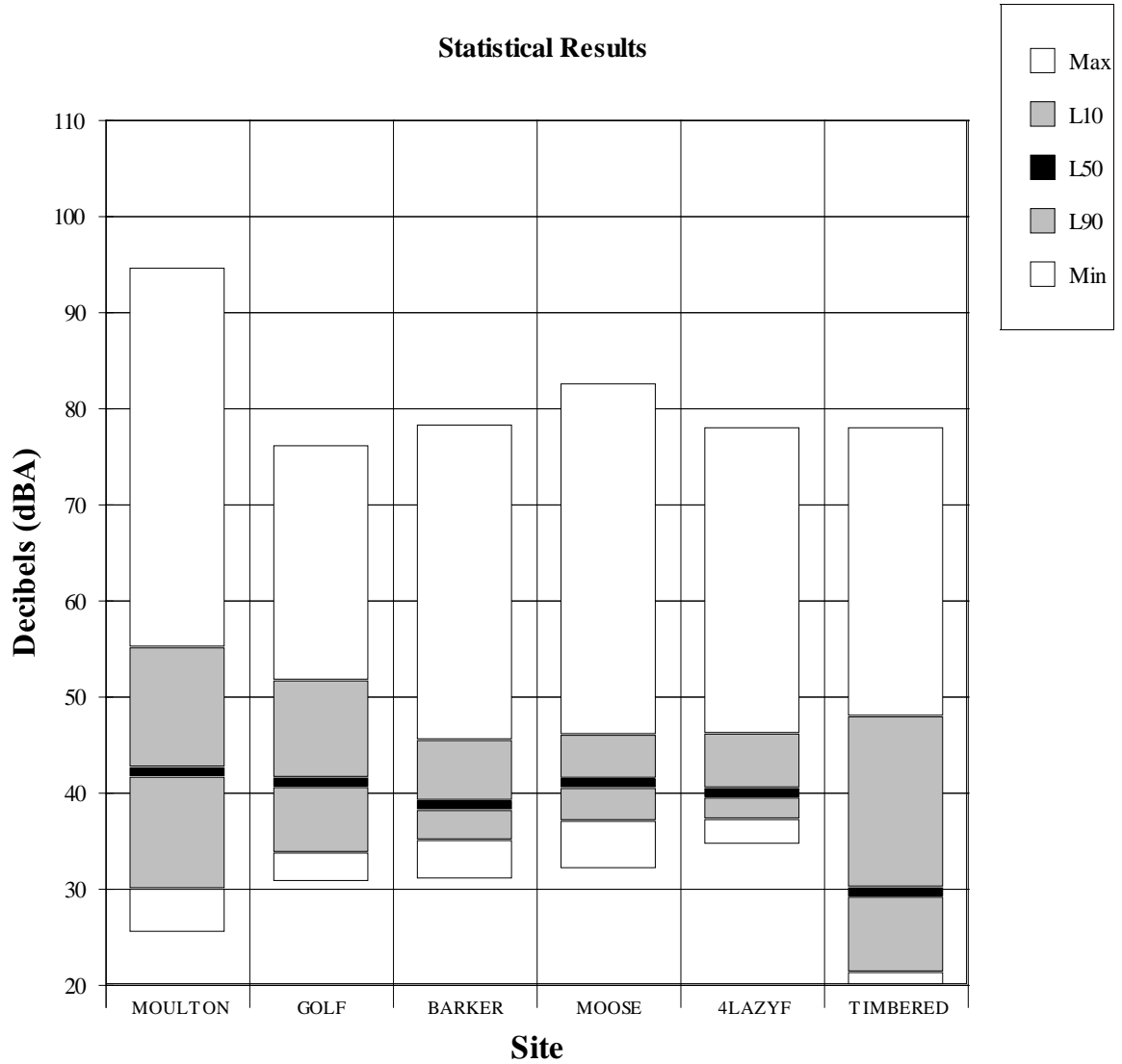
Figure 4-2 Ambient Noise Measurement Results for All Sites Jackson Hole Airport 2016 Annual Report Period: August 30, 2016 and September 12, 2016
