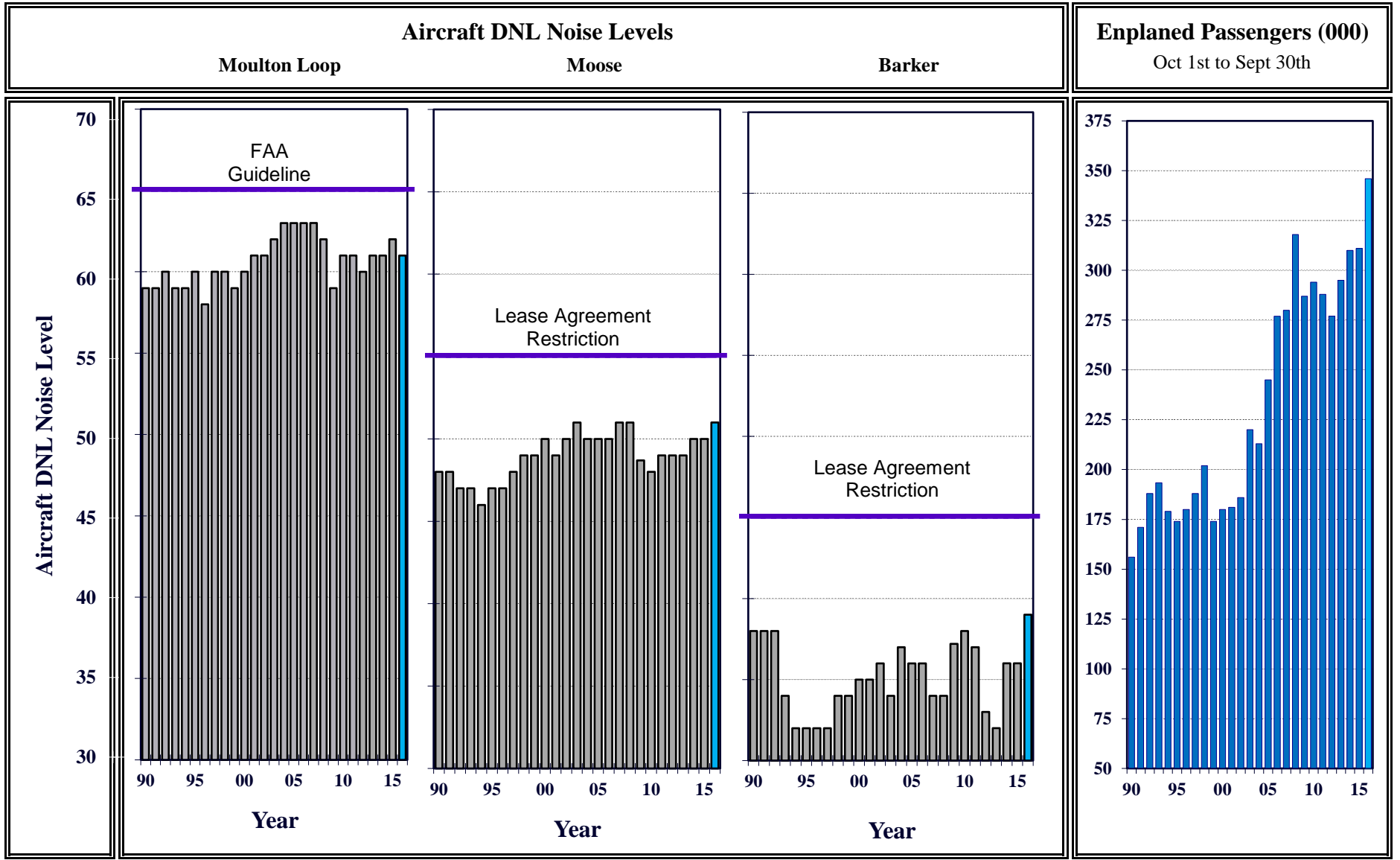
Figure 4-12 2016 Annual DNL Noise Report Jackson Hole Airport 2016 Annual Report October 1st 2015 to September 30th 2016
