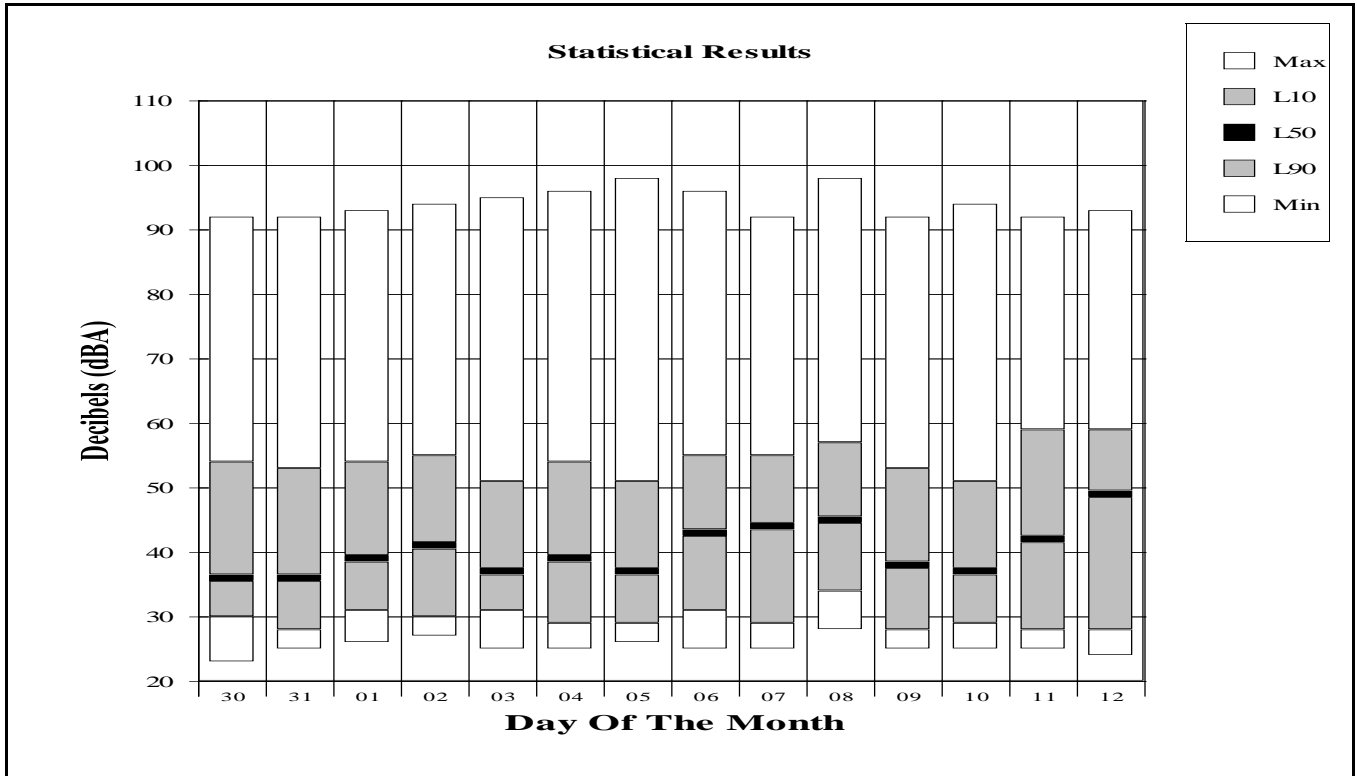
Figure 4-3 Site Specific Ambient Noise Measurement Results Jackson Hole Airport 2016 Annual Report Site: Moulton Loop
