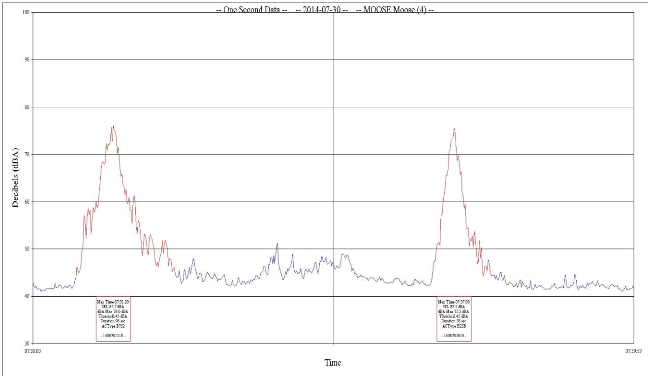
Figure 4-1 Sample Time History Noise Plot of Aircraft and Ambient Noise Jackson Hole Airport 2014 Annual Report Period: July 30, 2014 07:30:00 to July 30, 2014 07:39:59 Site: Moose (top) - 4 Lazy F Ranch (bottom)
