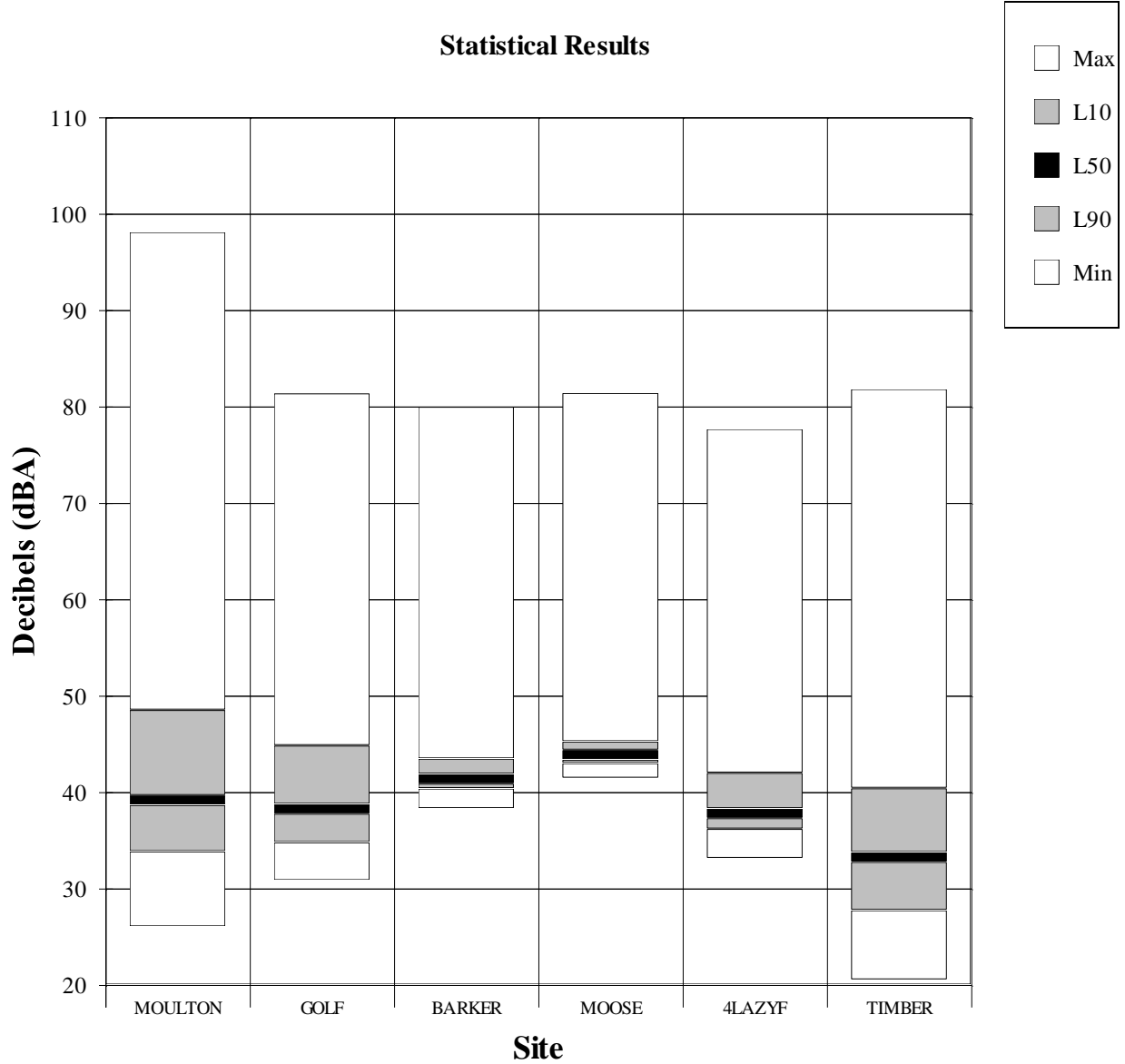
Figure 4-2 Ambient Noise Measurement Results for All Sites Jackson Hole Airport 2014 Annual Report Period: July 26, 2014 and August 10, 2014
