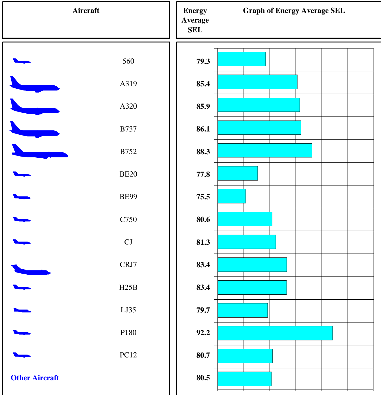
Figure 4-7 Single Event Noise Level by Aircraft Report Jackson Hole Airport 2014 Annual Report Period: July 26, 2014 to August 10, 2014 Site: Moose Operations: Arrivals Runway: 19 Tracks: ALL
