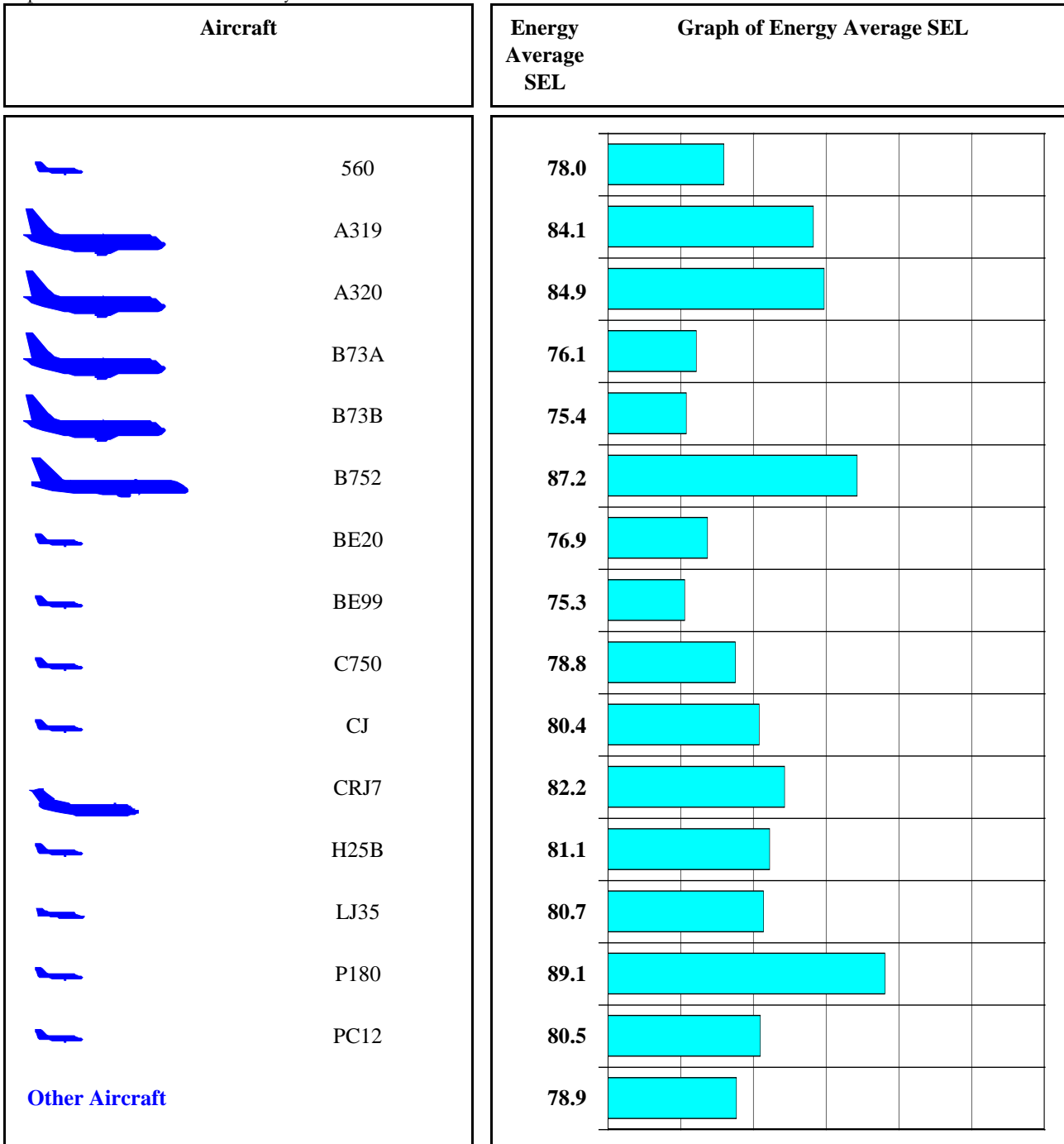
Figure 4-7 Single Event Noise Level by Aircraft Report Jackson Hole Airport 2013 Annual Report Period: August 2013 to September 2013 Site: Moose Operations: Arrivals Runway: 19 Tracks: ALL
