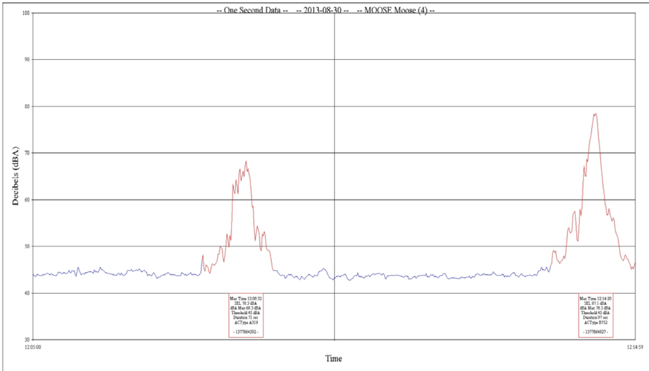
Figure 4-1 Sample Time History Noise Plot of Aircraft and Ambient Noise Jackson Hole Airport 2013 Annual Report Period: August 30, 2013 12:05:00 to August 30, 2013 12:14:59 Site: Moose (top) - 4 Lazy F Ranch (bottom)
