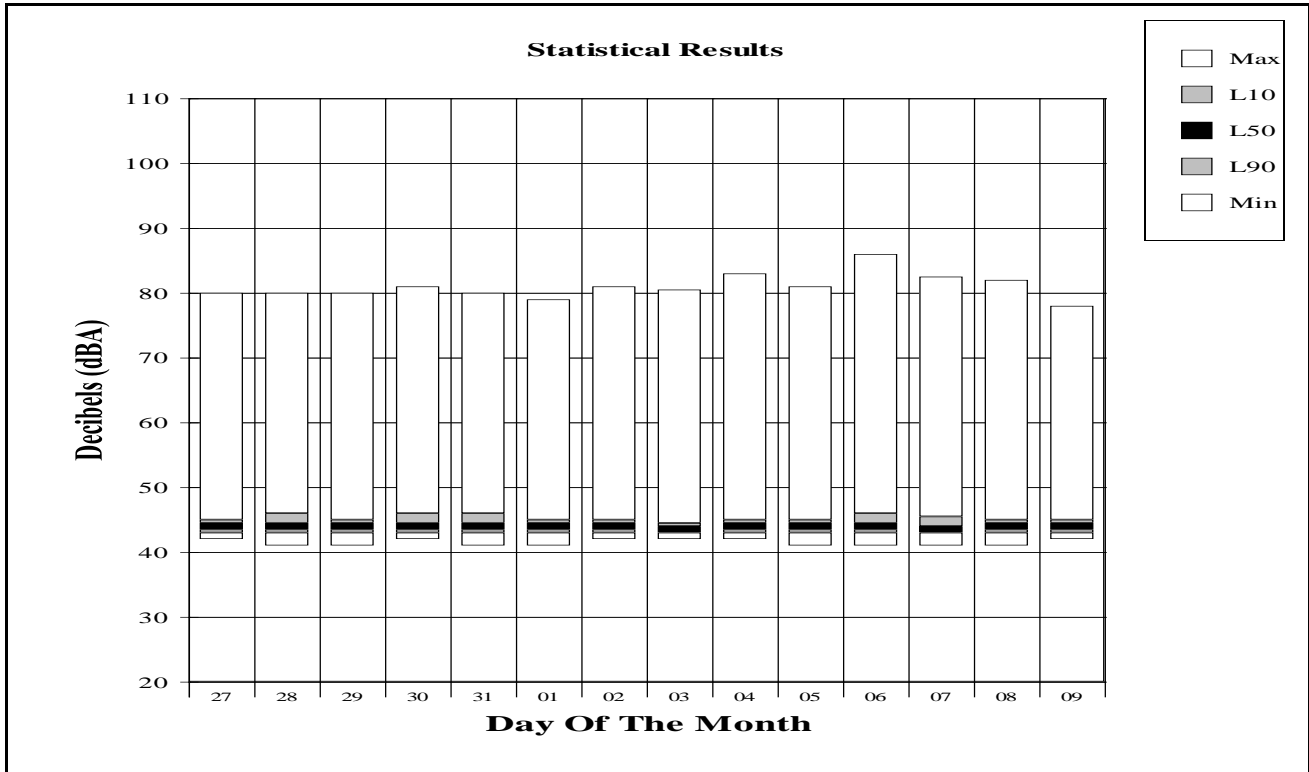
Figure 4-3 Site Specific Ambient Noise Measurement Results Jackson Hole Airport 2013 Annual Report Site: Moose
