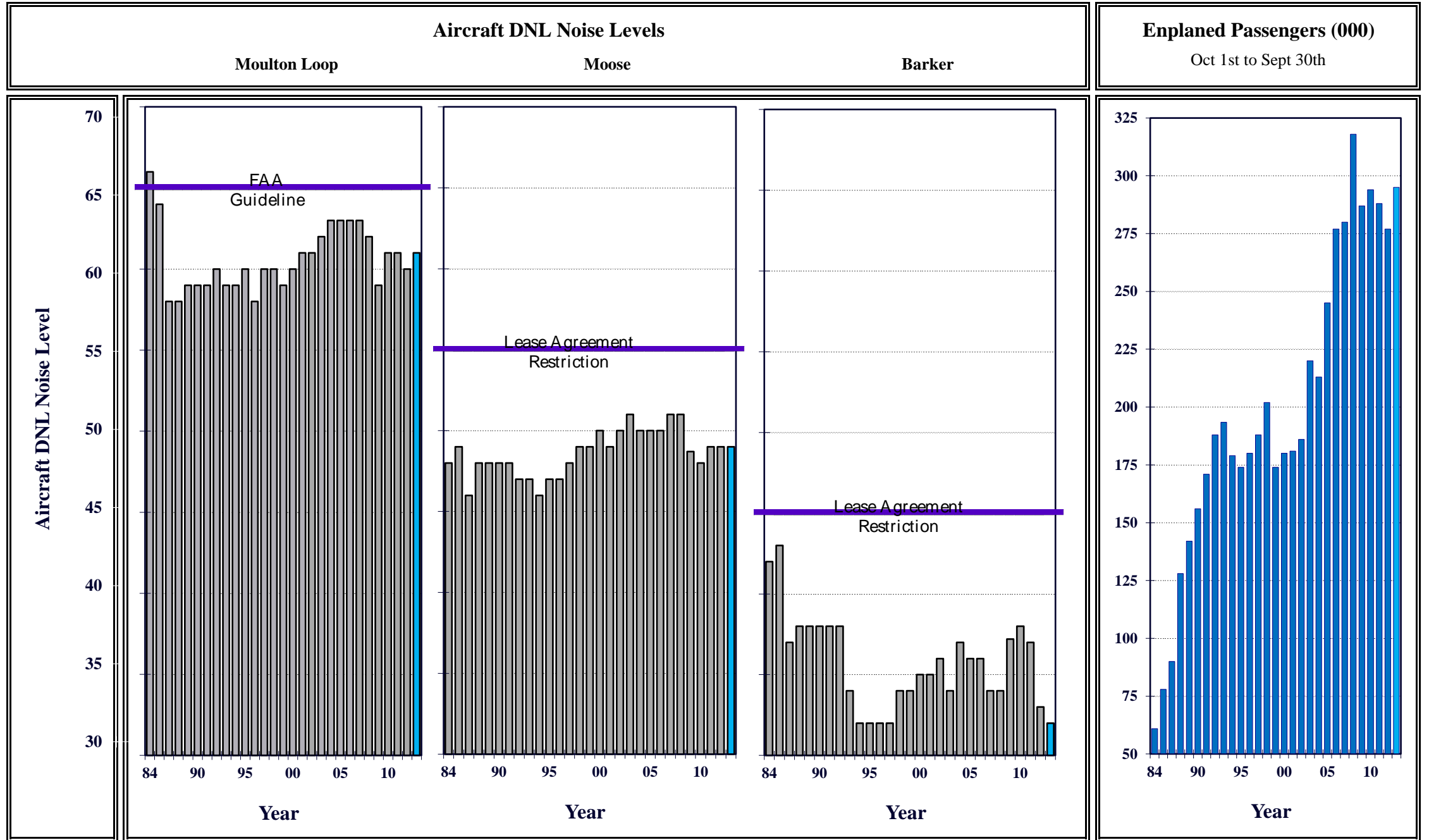
Figure 4-12 2010 Annual DNL Noise Report Jackson Hole Airport 2013 Annual Report October 1st 2012 to September 30th 2013
