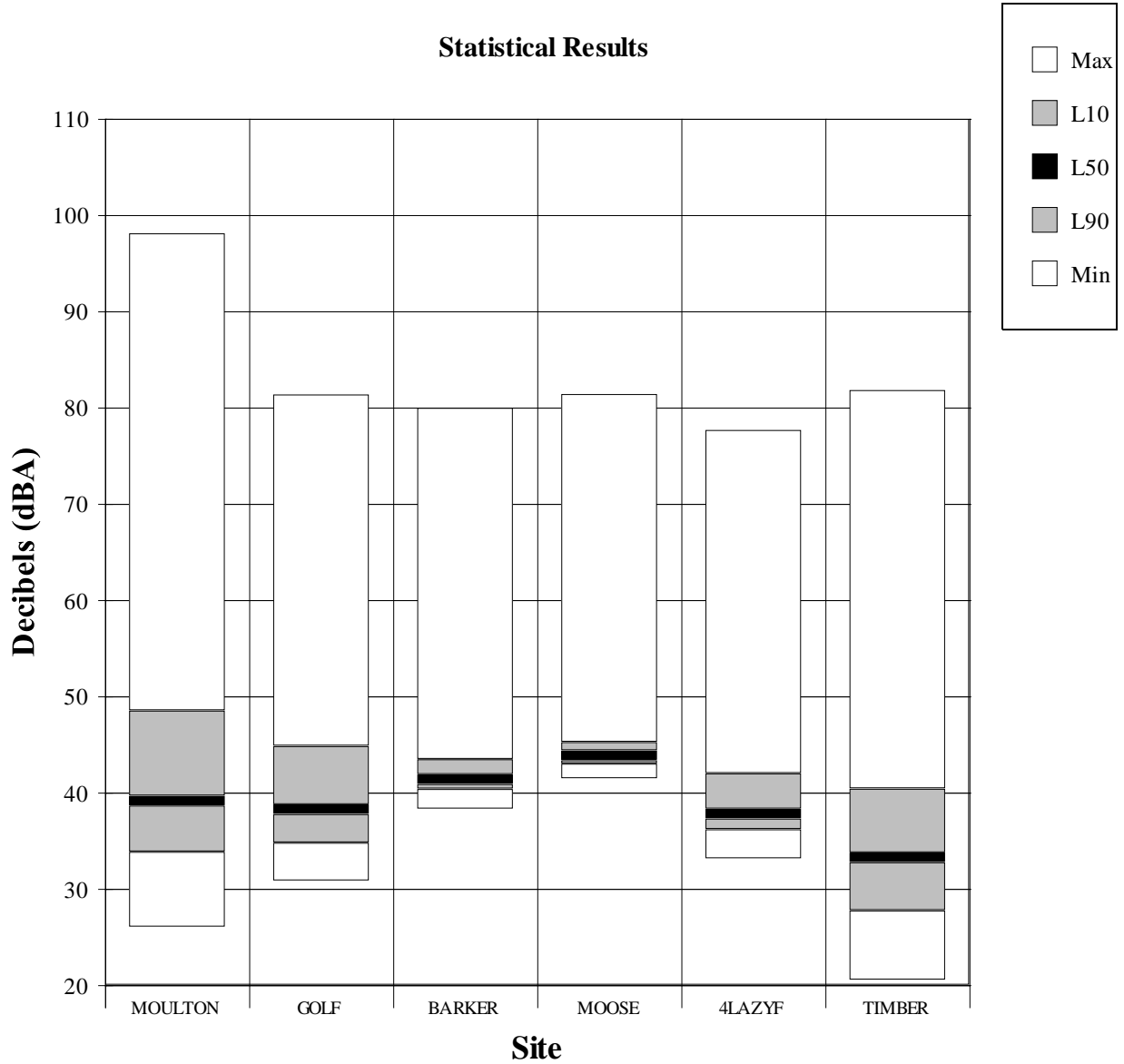
Figure 4-2 Ambient Noise Measurement Results for All Sites Jackson Hole Airport 2013 Annual Report Period: August 27, 2013 and September 9, 2013
