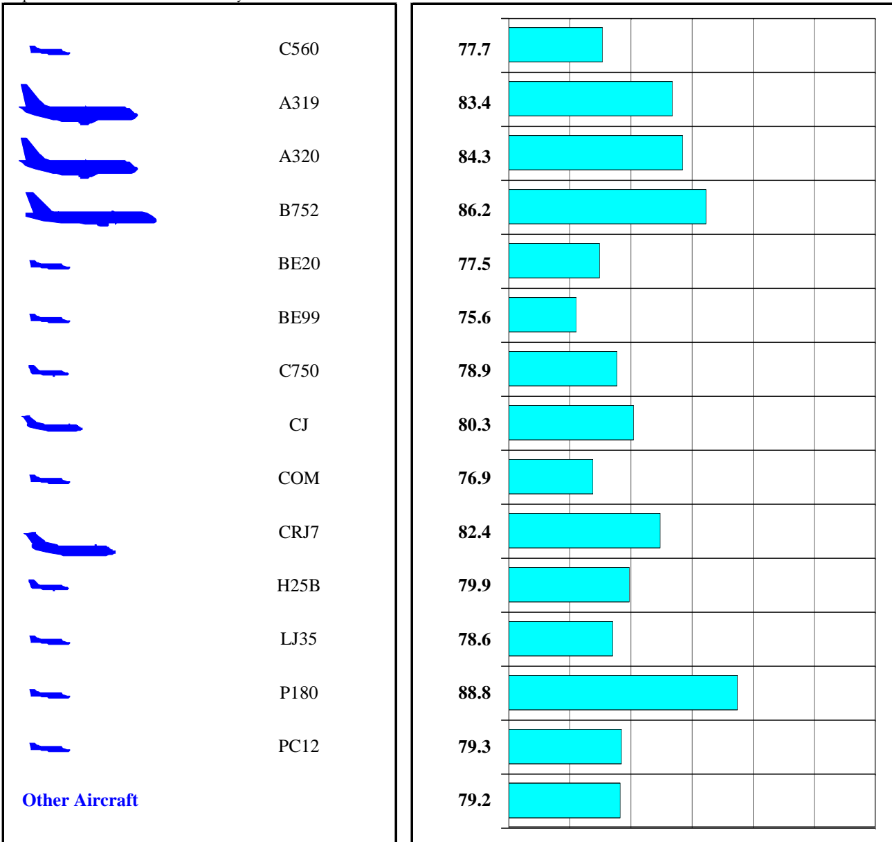
Figure 4-7 Single Event Noise Level by Aircraft Report Jackson Hole Airport 2011 Annual Report Period: August 2011 to September 2011 Site: Moose Operations: Arrivals Runway: 19 Tracks: ALL
