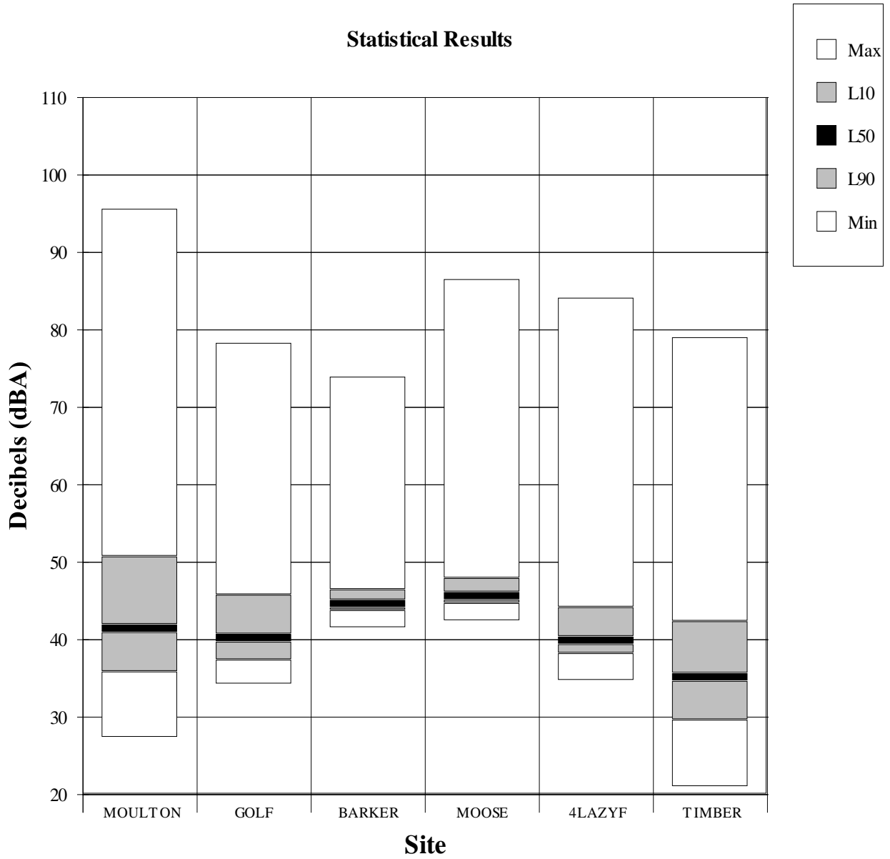
Figure 4-2 Ambient Noise Measurement Results for All Sites Jackson Hole Airport 2011 Annual Report Period: August 29, 2011 and September 11, 2011
