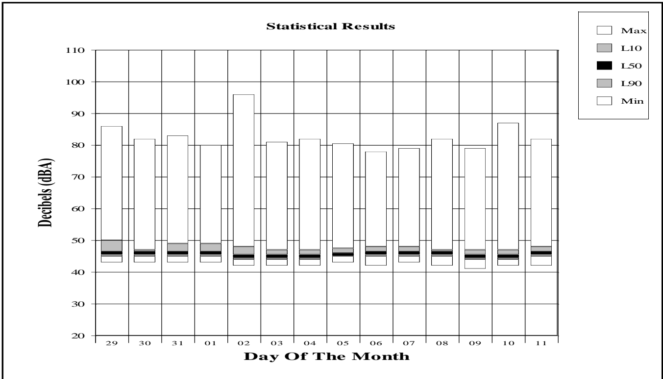
Figure 4-3 Site Specific Ambient Noise Measurement Results Jackson Hole Airport 2011 Annual Report Site: Moose
