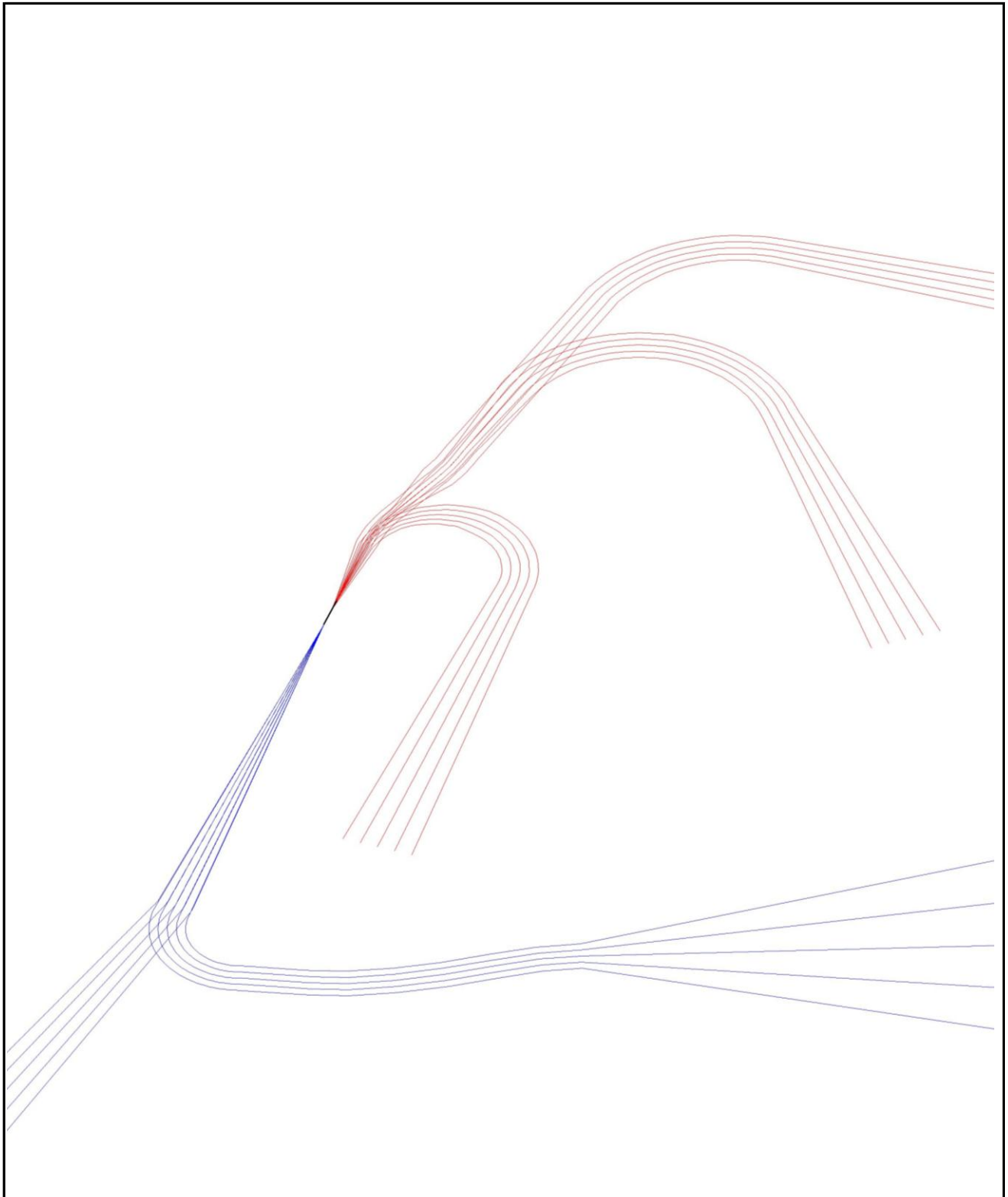
Figure 5-2 Flight Tracks for North Flow Jackson Hole Airport 2010 Annual Report Arrival and Departure Tracks for Runway 1
