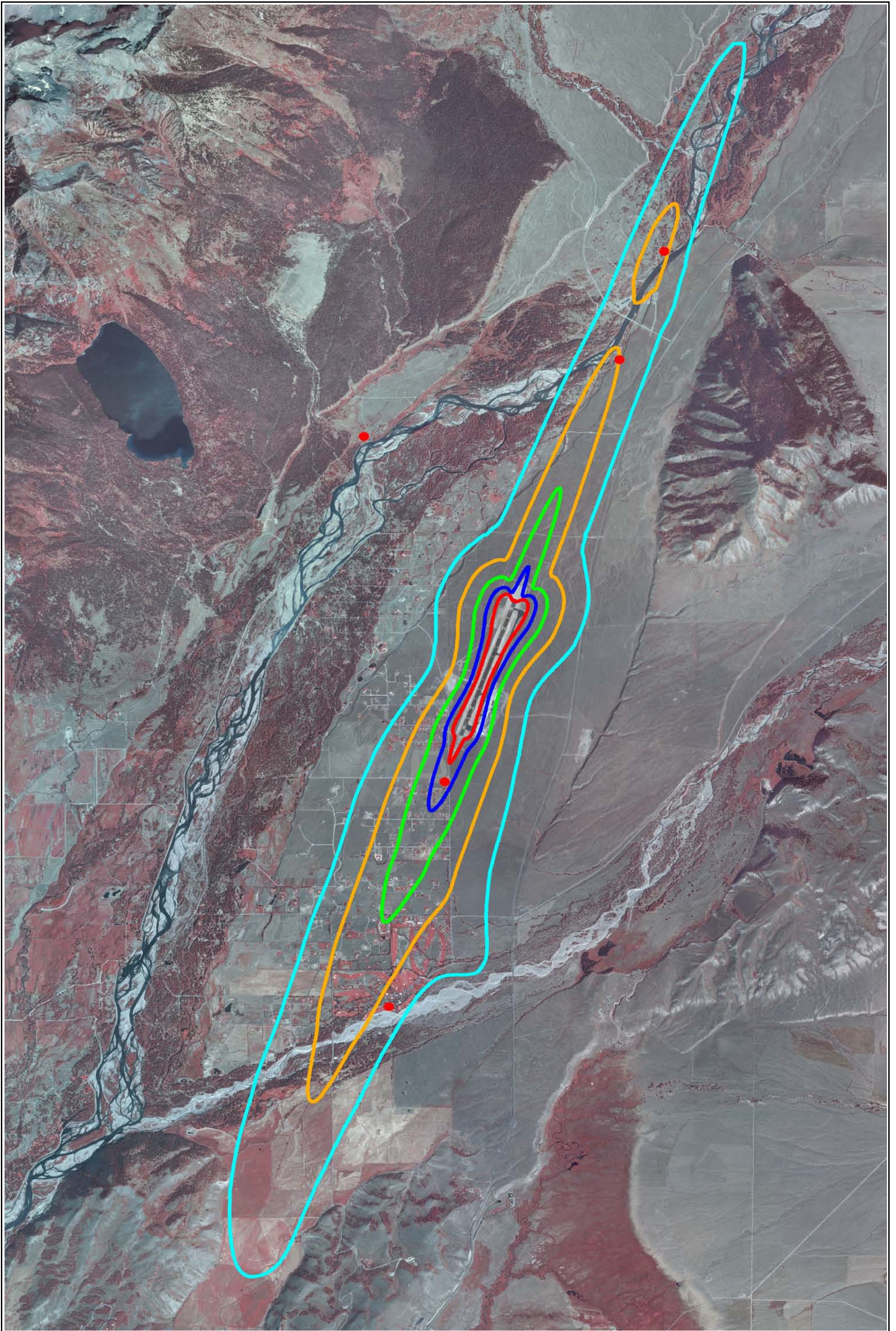
2010 ANNUAL DNL NOISE CONTOURS
