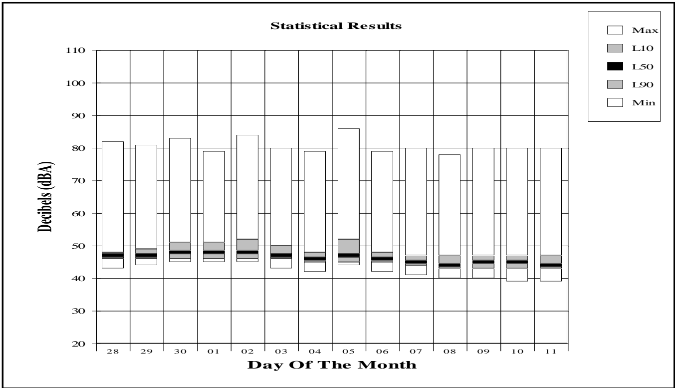
Figure 4-3 Site Specific Ambient Noise Measurement Results Jackson Hole Airport 2010 Annual Report Site: Moose
