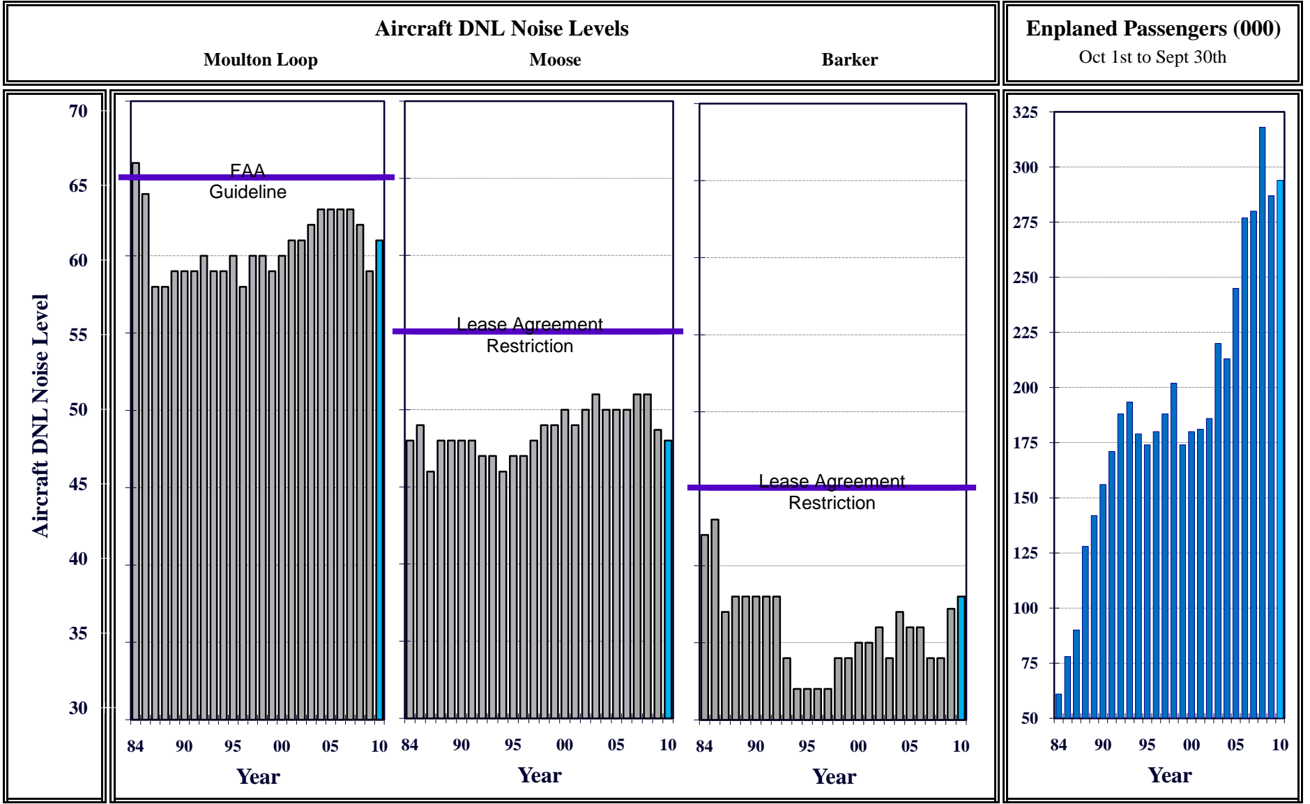
Figure 4-12 2010 Annual DNL Noise Report Jackson Hole Airport 2010 Annual Report October 1st 2009 to September 30th 2010
